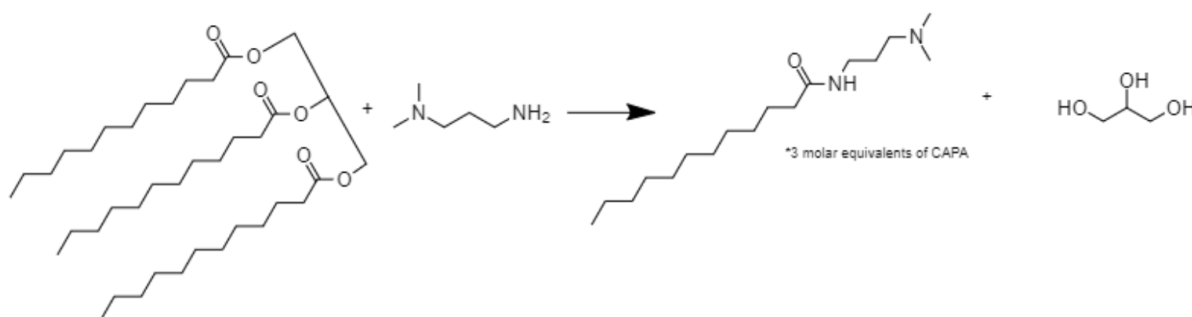
Figure 2: Reaction scheme for the production of cocoamidopropylamine (CAPA) from triglyceride (oil) and DMAPA using the C12 chain length as an example.
